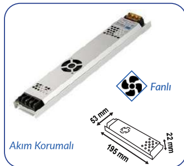
12V 16.5A 200W ULTRA SLİM TRAF0
