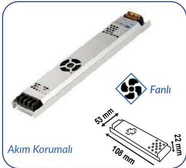
12V 5A 60W ULTRA SLİM TRAF0
