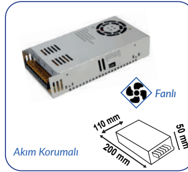
5V 60A 300W KALIN KASA TRAFİ
